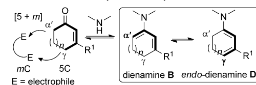
Scheme 1. Different aminocatalytic modes of cyclic enones.
